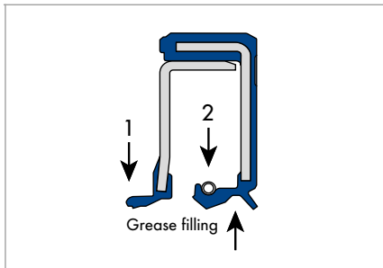
Simmerring MSS 1
